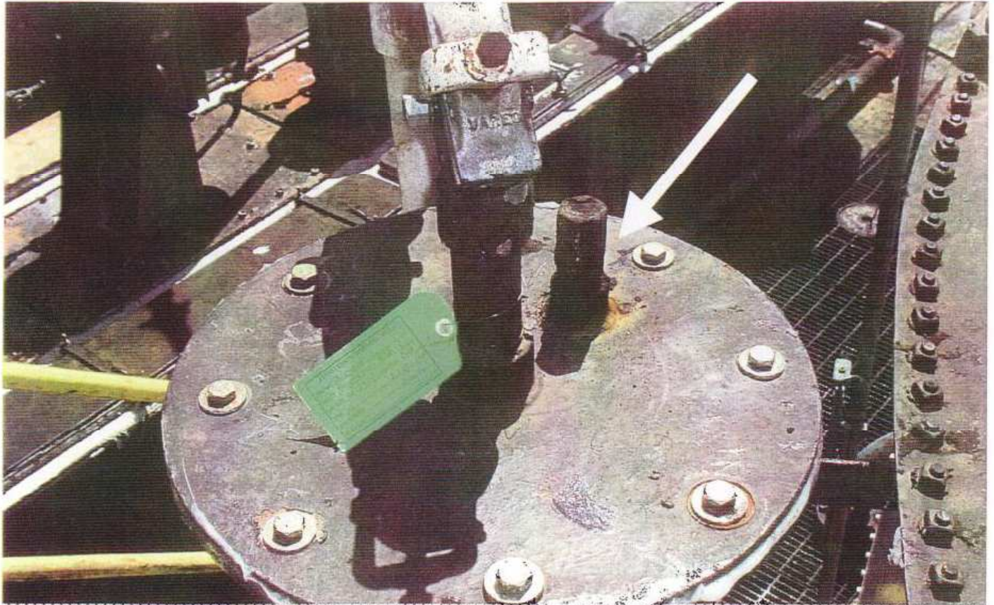
Photograph #9, taken 4/19/2003. The bull plug, as denoted by the arrow, was resting on top of an open threaded connection, allowing VOC emissions from Flange #1412, which is at the top of the external water level boot of the water injection tank.
