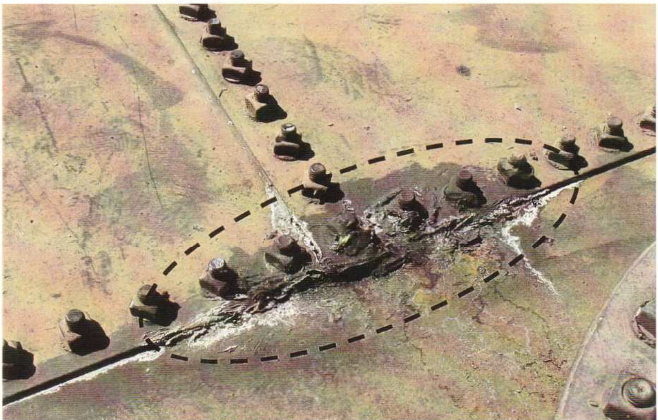
Photograph #8, taken 4/19/2003. Location of vapor leak at the overlap of three bolted plates on the roof of the water injection tank (Item #6, Permit R-D93078, A/N 306537)
